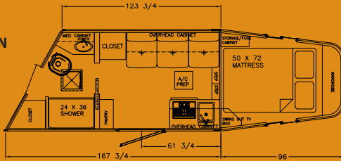
10' PKG. B FLOORPLAN
