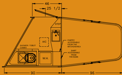
4' FLOORPLAN
