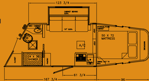
10' PKG. B FLOORPLAN
