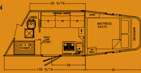
8' FLOORPLAN
